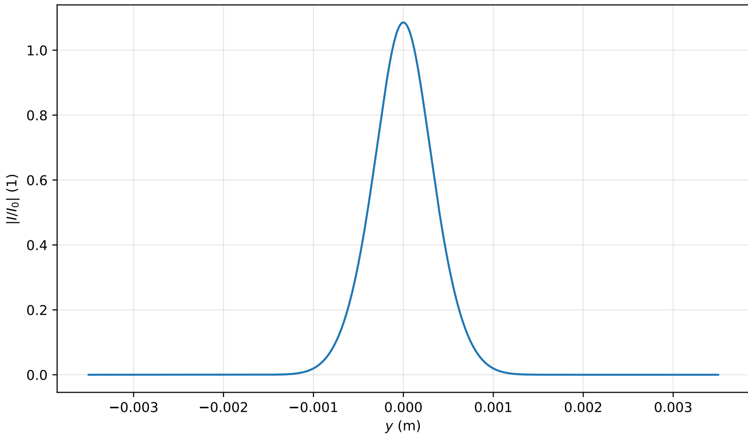
Intensity profile I(x=0, y, z=0.478)/I_0 , \text{Pin}=0.7\text{Pcr} , artificial time
